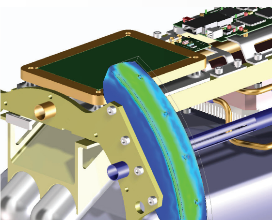
Simulate and analyze designs under stress and thermal conditions with Finite Element Analysis.
